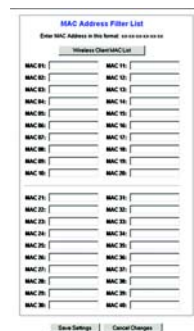
Figure 5-17: MAC Address Filter List
